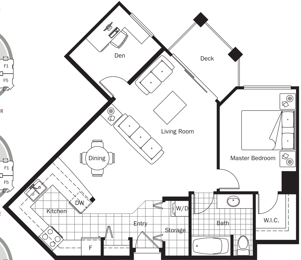
BUILDING B FIRST FLOOR
